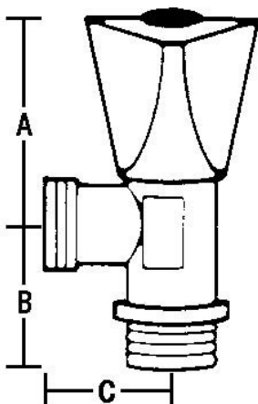
79 Angle valve
