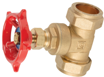
L197 Brass Gate Valve CxC
